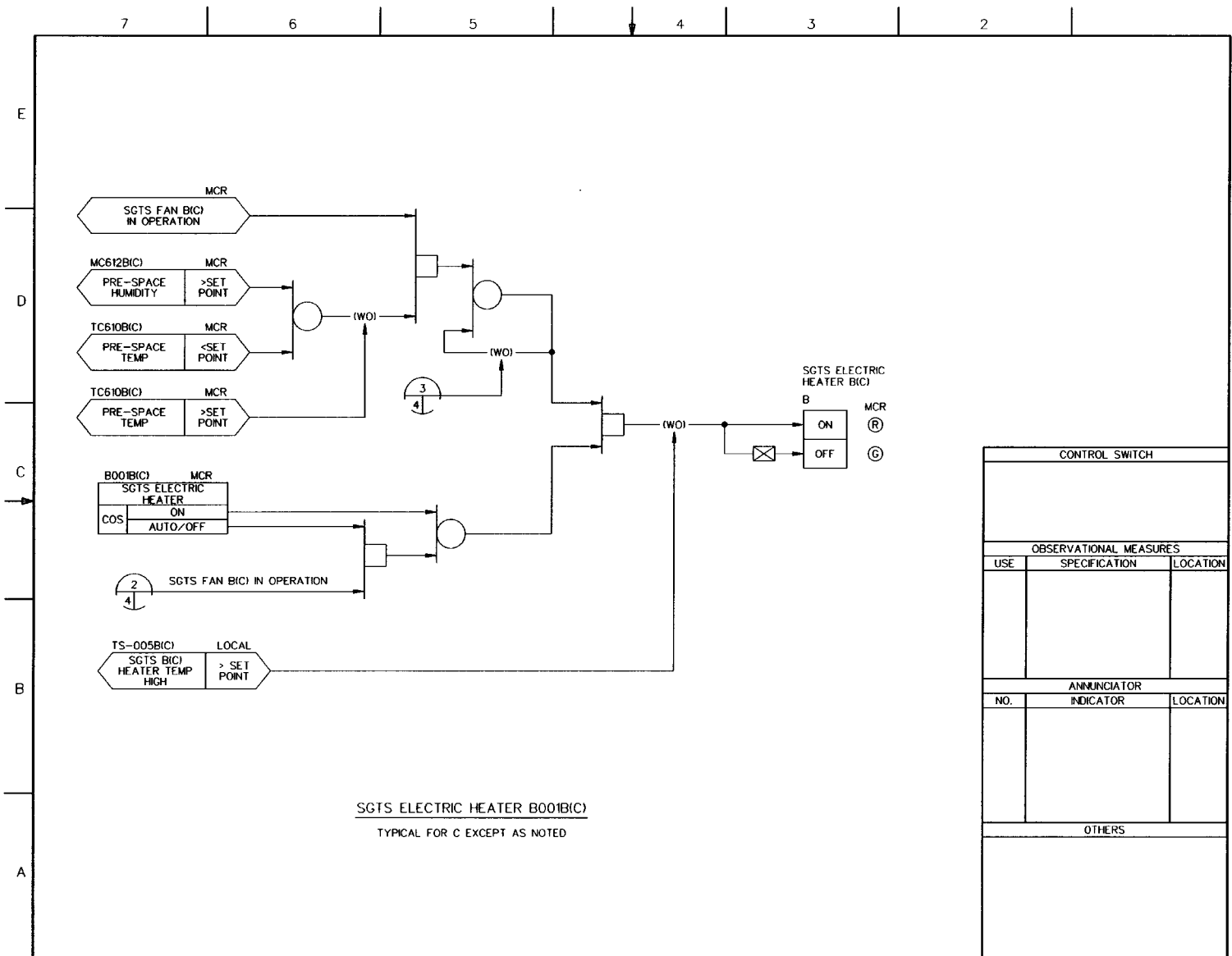
FIGURE 7.3-6 STANDBY GAS TREATMENT SYSTEM IBD (Sheet 5 of 10) ABWR DCD/Tier 2 Rev. 0 21-233
