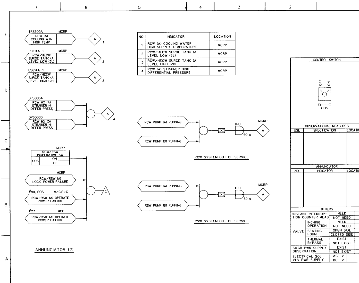
FIGURE 7.3-7 REACTOR BUILDING COOLING WATER/REACTOR SERVICE WATER SYSTEM IBD (Sheet 17 of 19)
