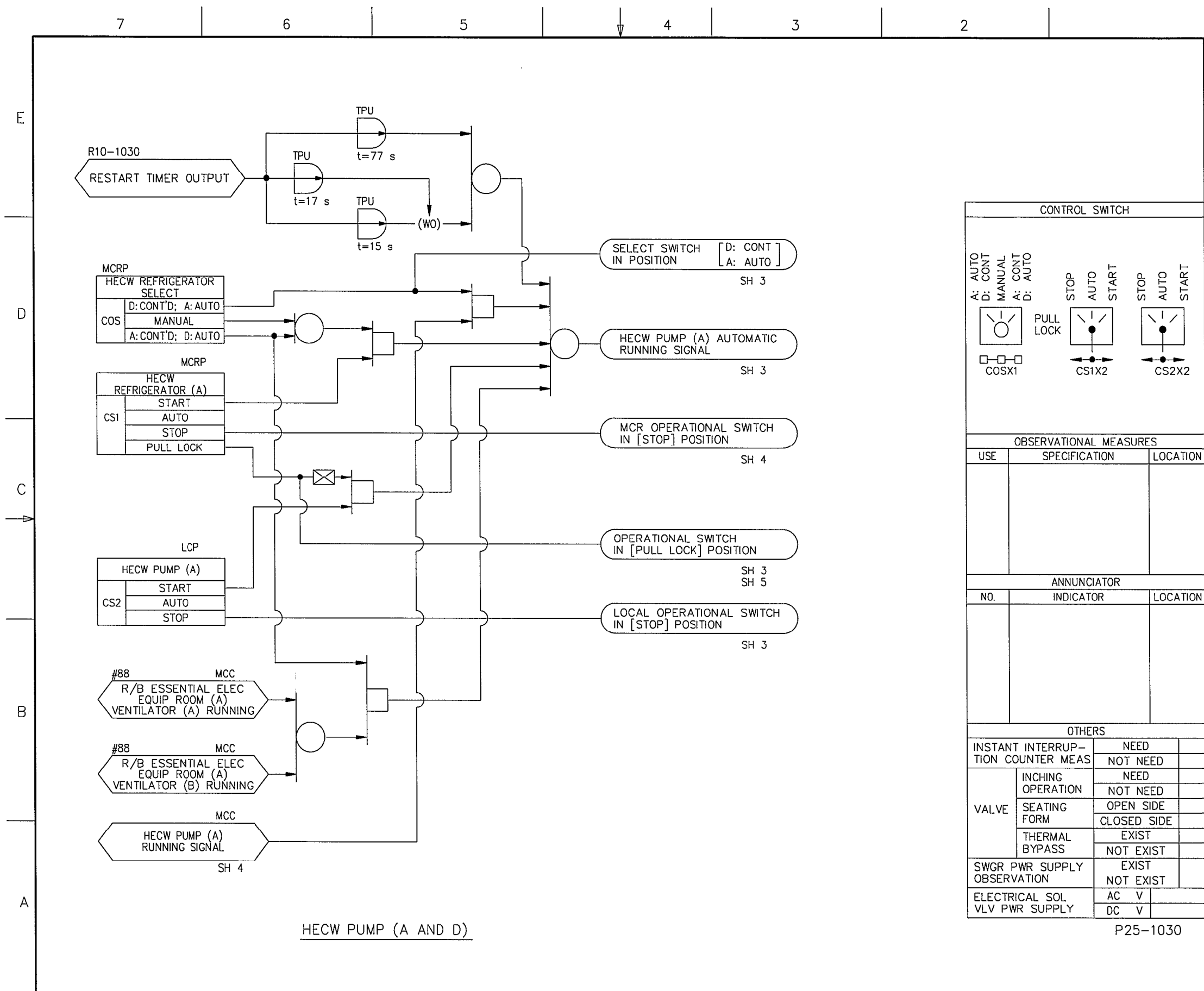
FIGURE 7.3-9 HVAC EMERGENCY COOLING WATER SYSTEM IBD (Sheet 2 of 11)
