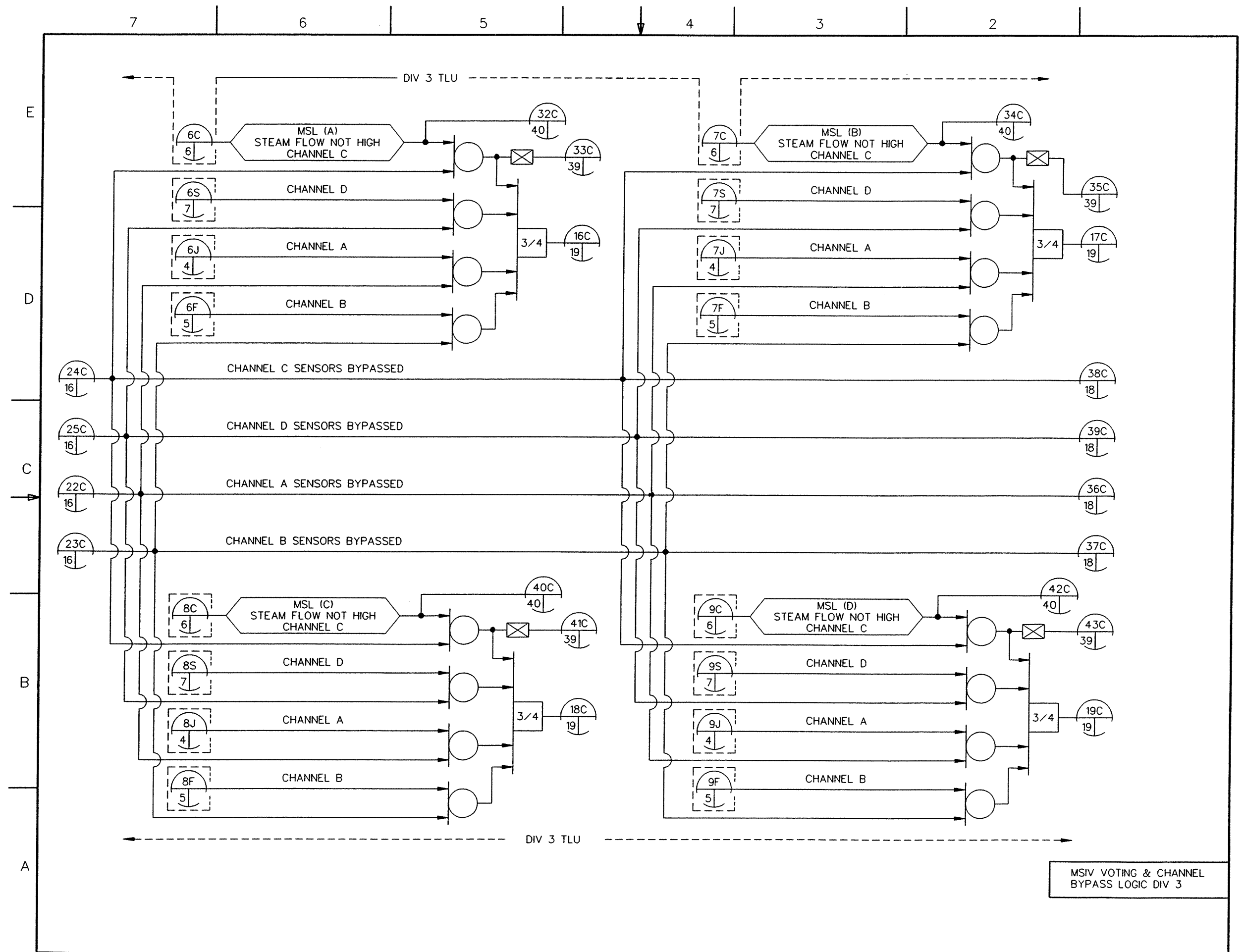
FIGURE 7.3-5 LEAK DETECTION AND ISOLATION SYSTEM IBD (Sheet 17 of 77)
