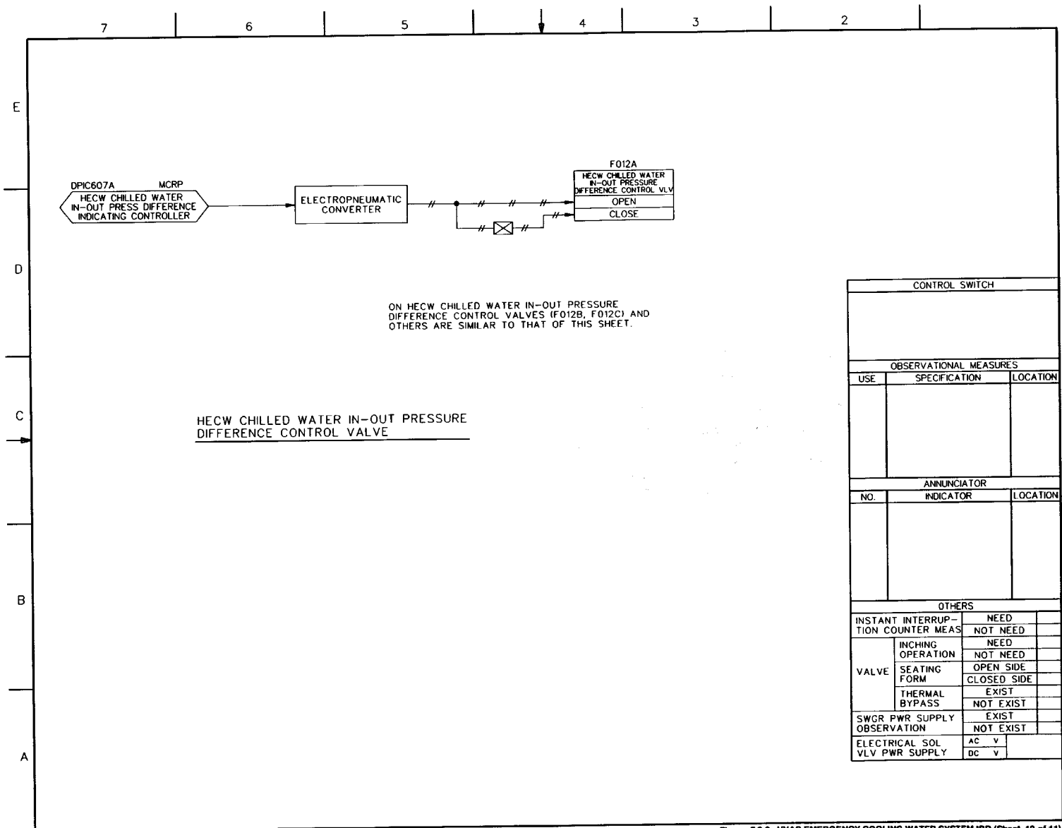
Figure 7.3-9 HVAC EMERGENCY COOLING WATER SYSTEM IBD (Sheet 10 of 11) ABWR DCD/Tier 2 Rev. 0 21-268
