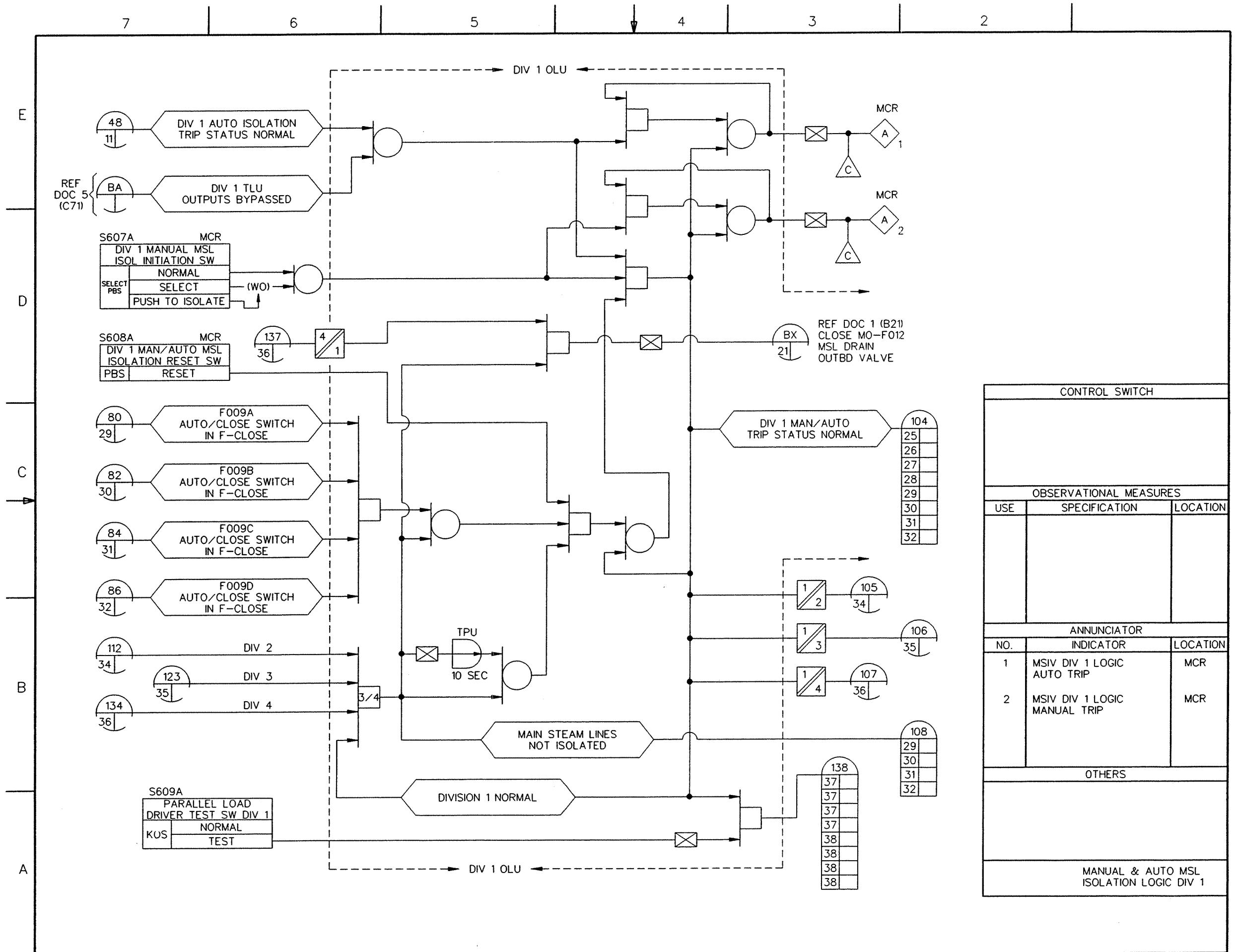
FIGURE 7.3-5 LEAK DETECTION AND ISOLATION SYSTEM IBD (Sheet 33 of 77)
