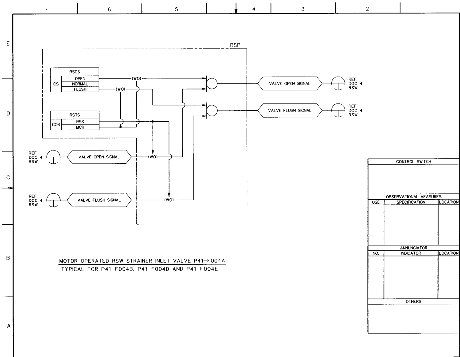
FIGURE 7.4-3 REMOTE SHUTDOWN SYSTEM IBD (Sheet 26 of 27) ABWR DCD/Tier 2 Rev. 0 21-305
