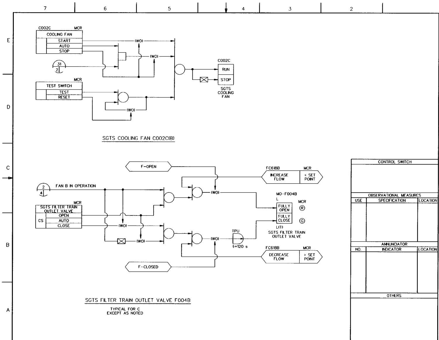
FIGURE 7.3-6 STANDBY GAS TREATMENT SYSTEM IBD (Sheet 3 of 11)
