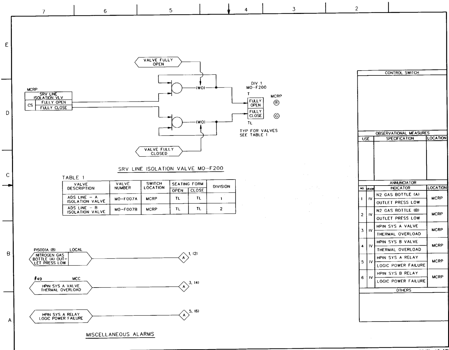
Figure 7.3-10 HIGH PRESSURE NITROGEN GAS SYSTEM IBD (Sheet 2 of 3) ABWR DCD/Tier 2 Rev. 0 21-271
