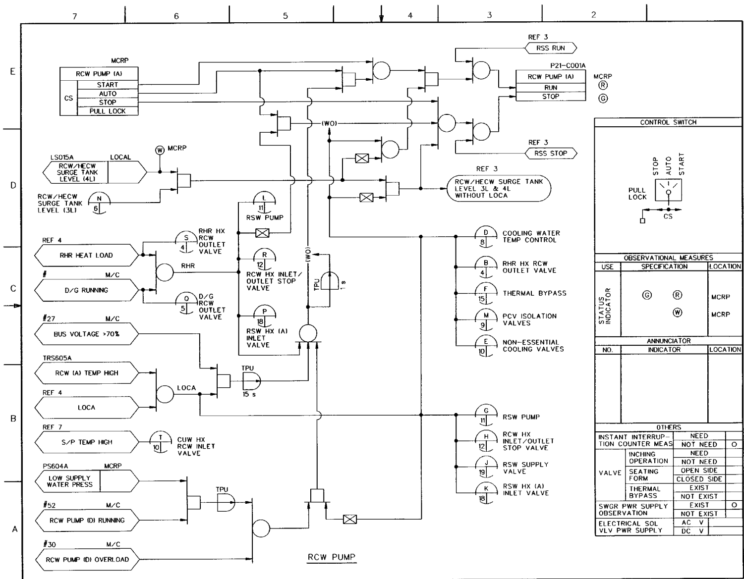
FIGURE 7.3-7 REACTOR BUILDING COOLING WATER/REACTOR SERVICE WATER SYSTEM IBD (Sheet 2 of 19)
