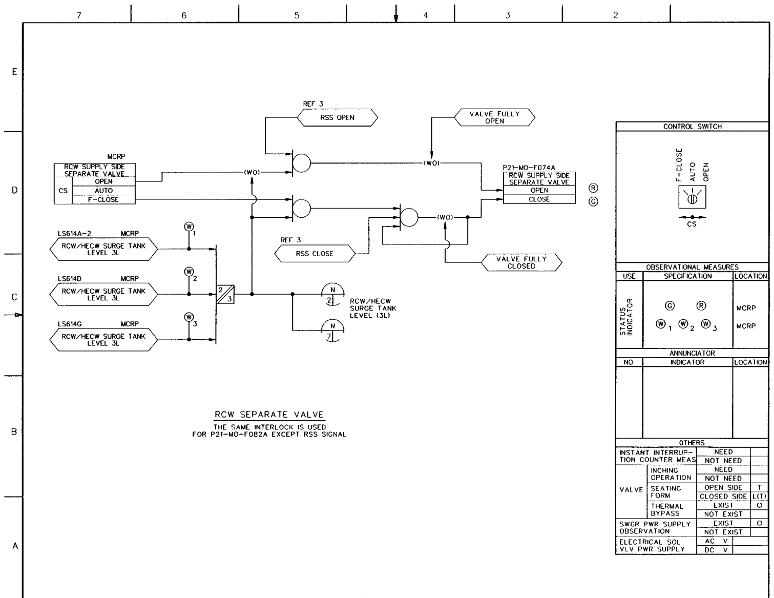
FIGURE 7.3-7 REACTOR BUILDING COOLING WATER/REACTOR SERVICE WATER SYSTEM IBD (Sheet 6 of 19)
