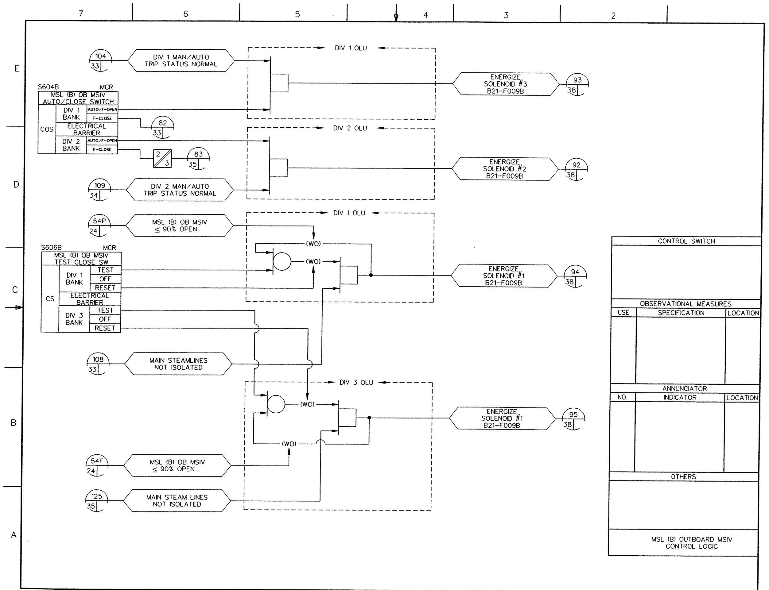
FIGURE 7.3-5 LEAK DETECTION AND ISOLATION SYSTEM IBD (Sheet 30 of 77)
