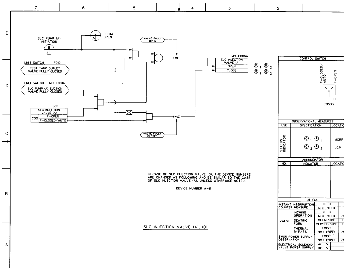
Figure 7.4-1 STANDBY LIQUID CONTROL SYSTEM IBD (Sheet 4 of 6) ABWR DCD/Tier 2 Rev. 0 21-276
