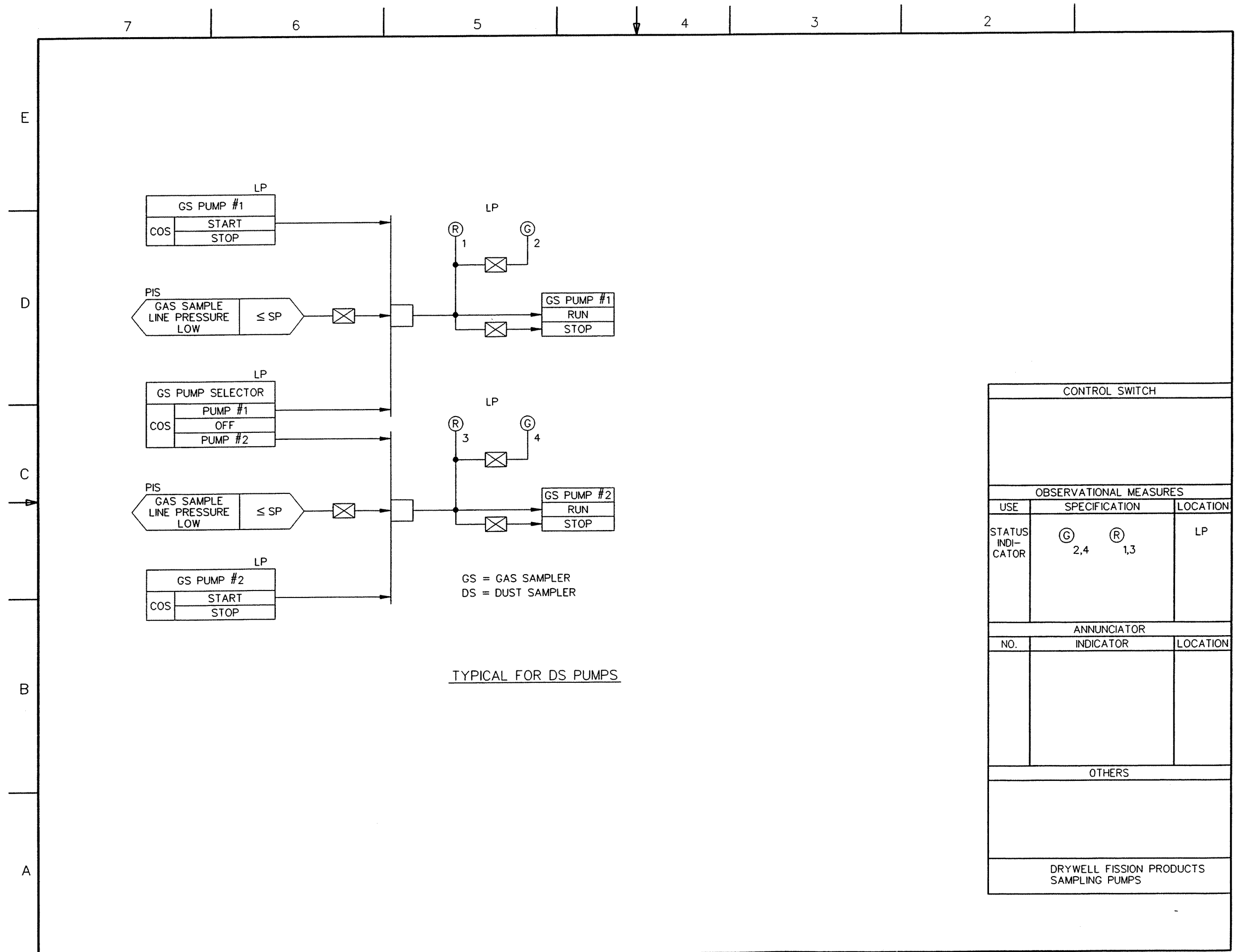
FIGURE 7.3-5 LEAK DETECTION AND ISOLATION SYSTEM IBD (Sheet 66 of 77) ABWR DCD/Tier 2 Rev. 0 21-228.66
