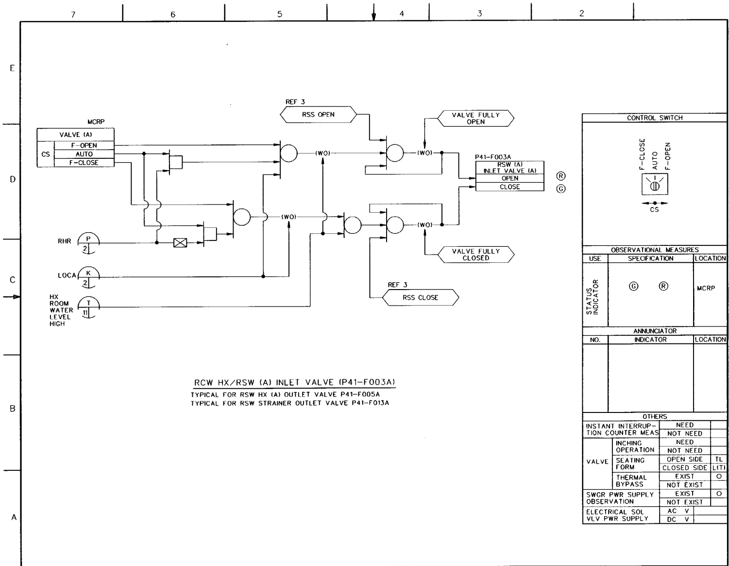
FIGURE 7.3-7 REACTOR BUILDING COOLING WATER/REACTOR SERVICE WATER SYSTEM IBD (Sheet 18 of 19) ABWR DCD/Tier 2 Rev. 0 21-257
