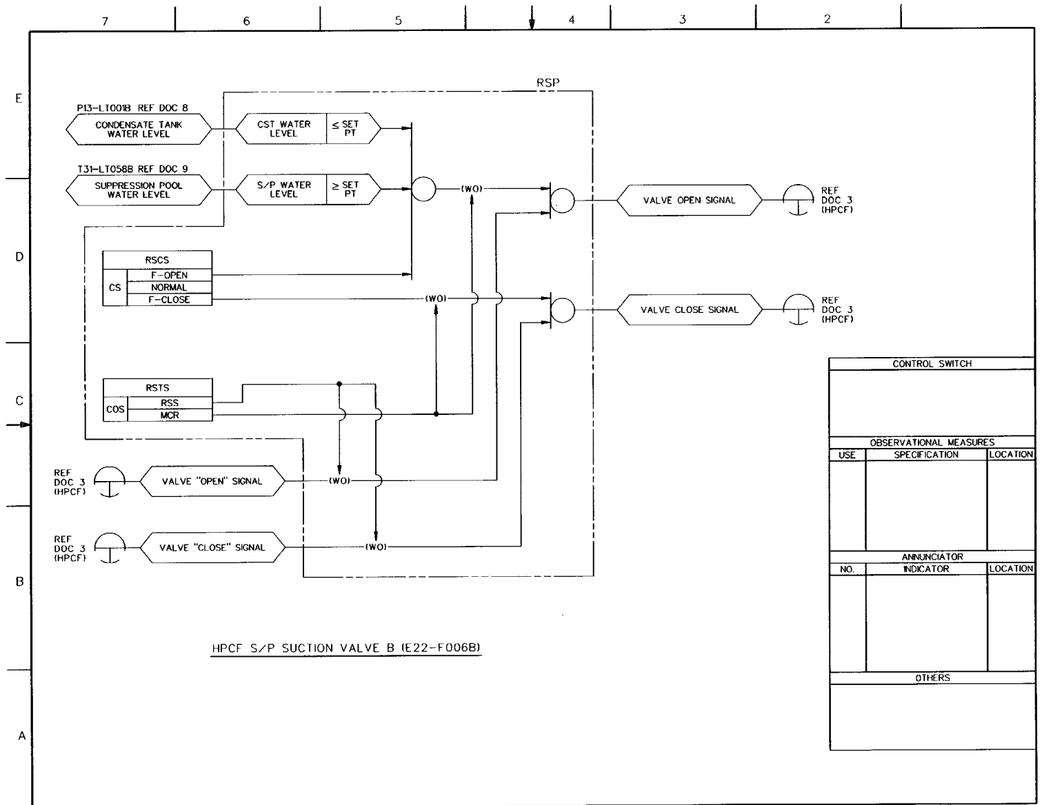
FIGURE 7.4-3 REMOTE SHUTDOWN SYSTEM IBD (Sheet 20 of 27)
