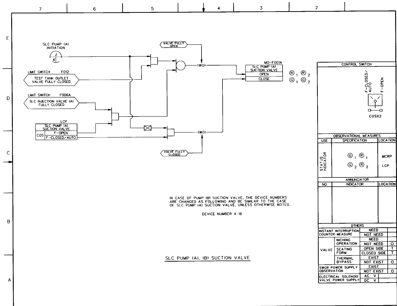
Figure 7.4-1 STANDBY LIQUID CONTROL SYSTEM IBD (Sheet 5 of 6) ABWR DCD/Tier 2 Rev. 0 21-277
