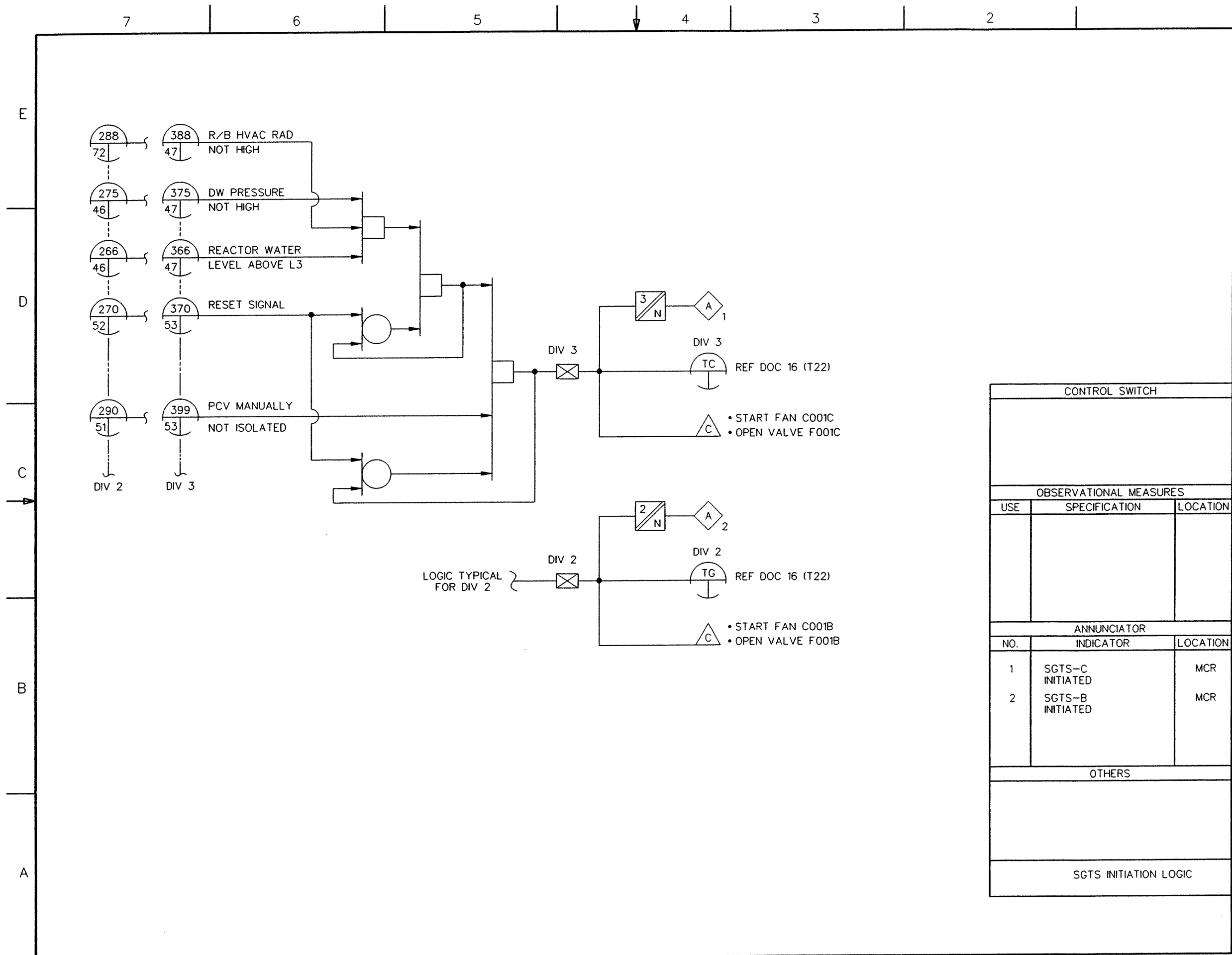
FIGURE 7.3-5 LEAK DETECTION AND ISOLATION SYSTEM IBD (Sheet 73 of 77) ABWR DCD/Tier 2 Rev. 0 21-228.73
