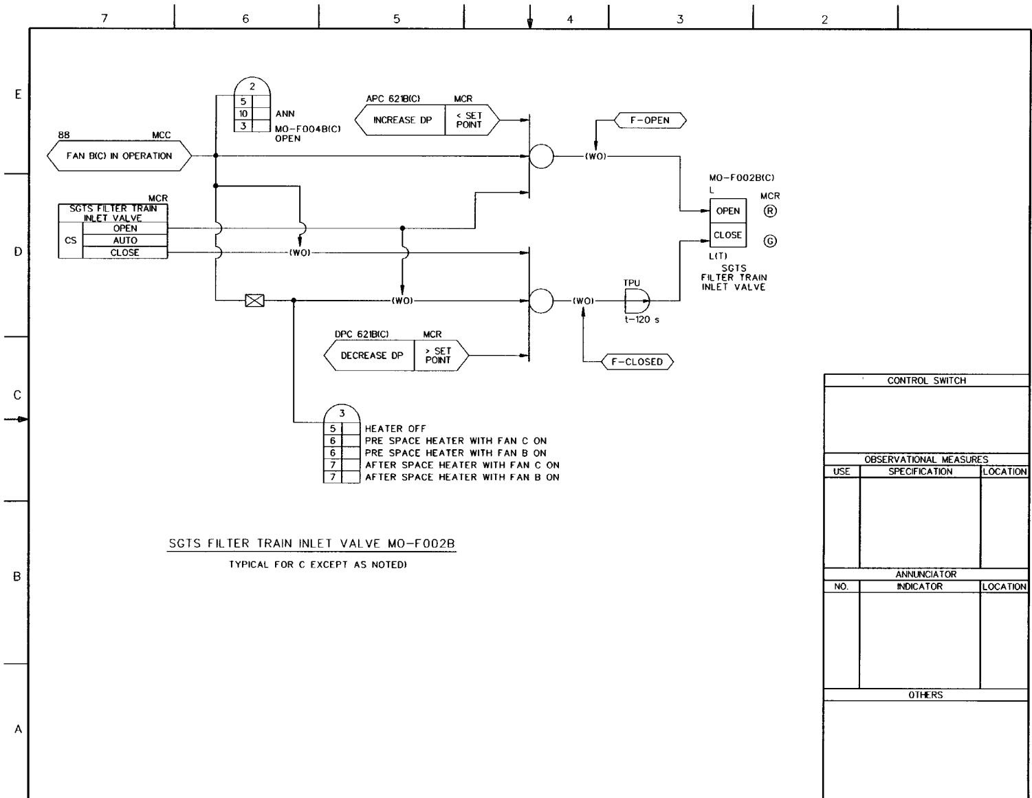
FIGURE 7.3-6 STANDBY GAS TREATMENT SYSTEM IBD (Sheet 4 of 10) ABWR DCD/Tier 2 Rev. 0 21-232
