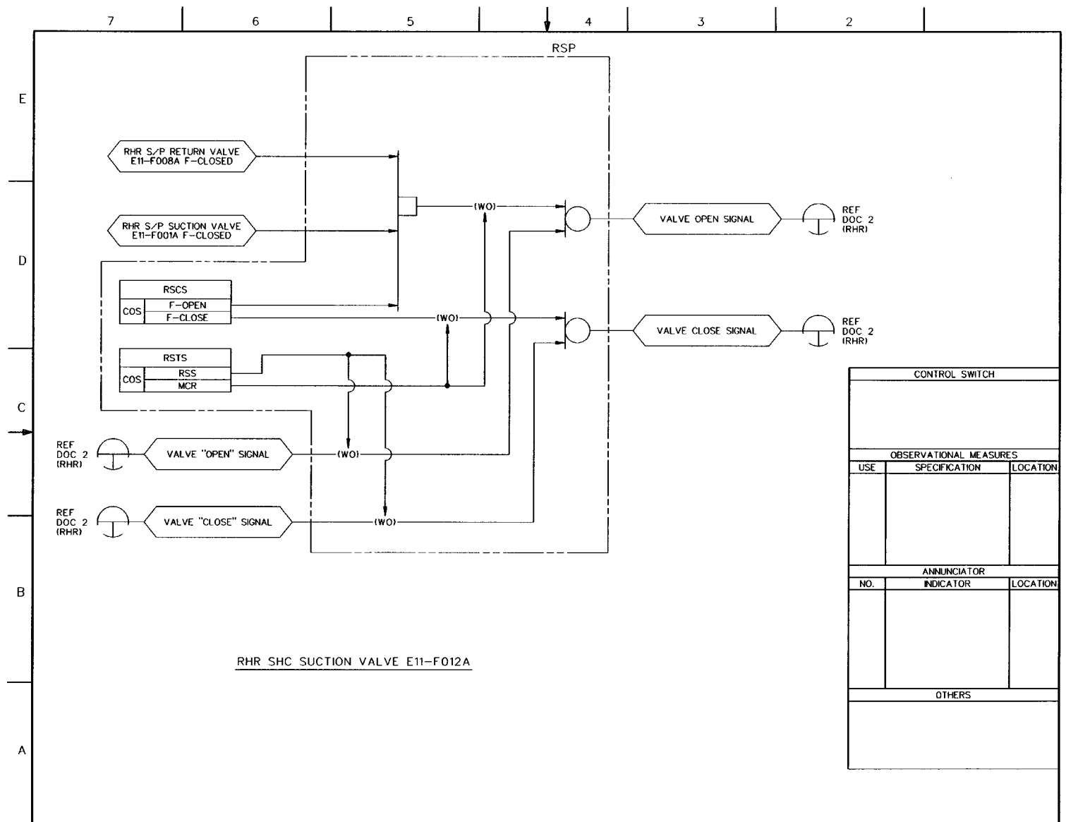
FIGURE 7.4-3 REMOTE SHUTDOWN SYSTEM (Sheet 17 of 27) ABWR DCD/Tier 2 Rev. 0 21-296
