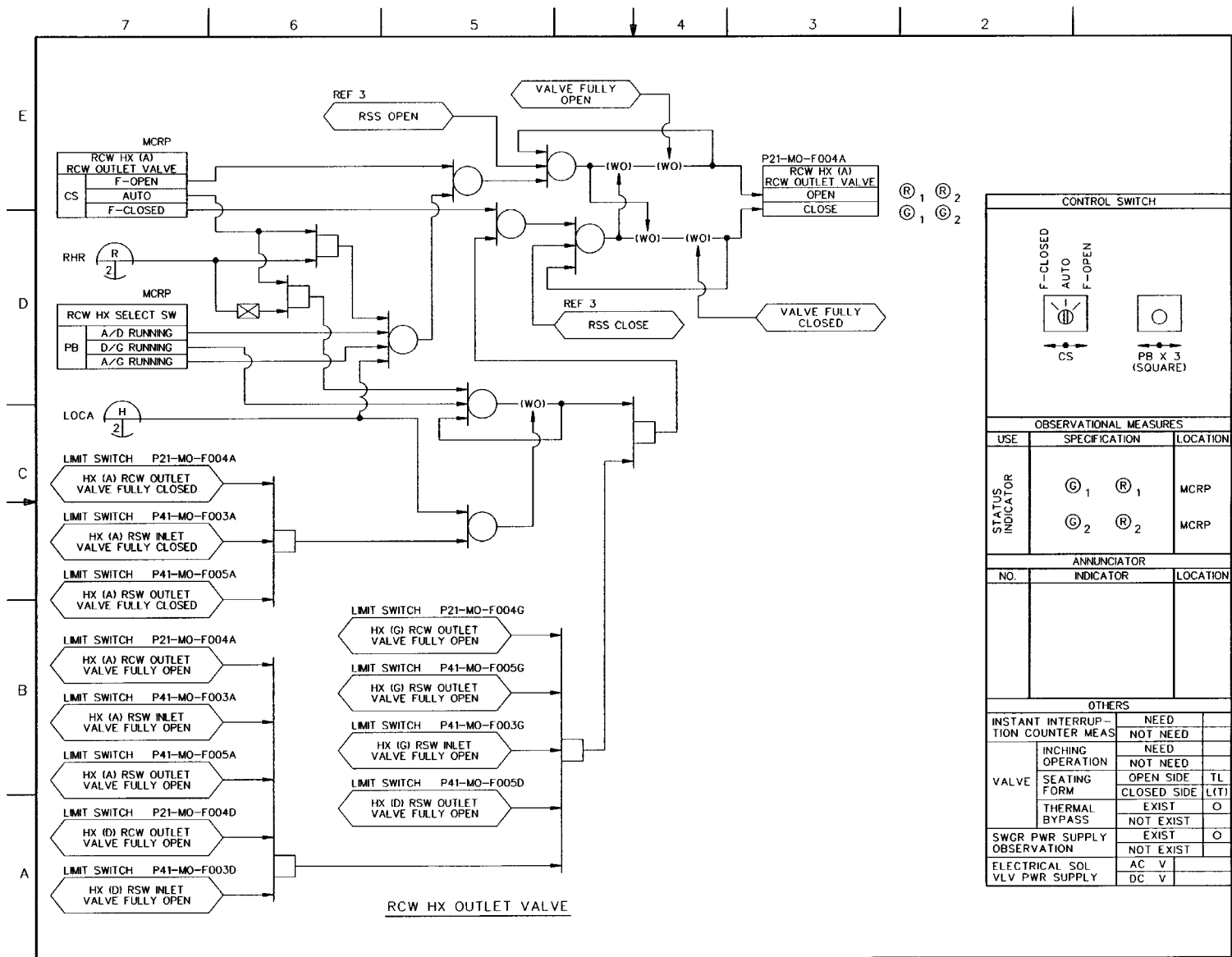
FIGURE 7.3-7 REACTOR BUILDING COOLING WATER/REACTOR SERVICE WATER SYSTEM IBD (Sheet 12 of 19) ABWR DCD/Tier 2 Rev. 0 21-251
