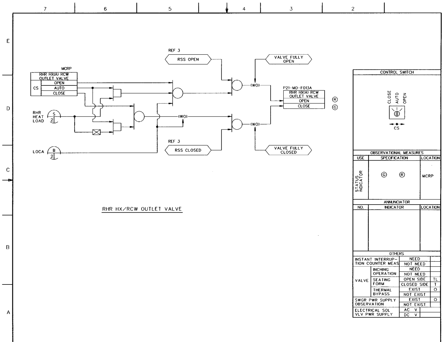
FIGURE 7.3-7 REACTOR BUILDING COOLING WATER/REACTOR SERVICE WATER SYSTEM IBD (Sheet 4 of 19)
