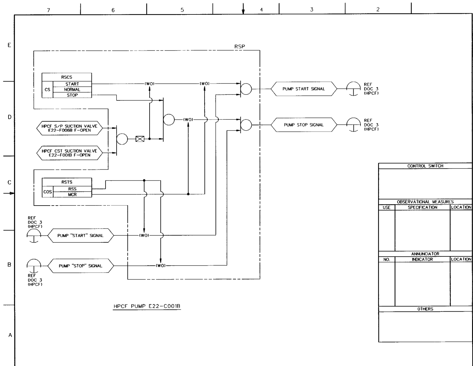
FIGURE 7.4-3 REMOTE SHUTDOWN SYSTEM IBD (Sheet 19 of 27) ABWR DCD/Tier 2 Rev. 0 21-298
