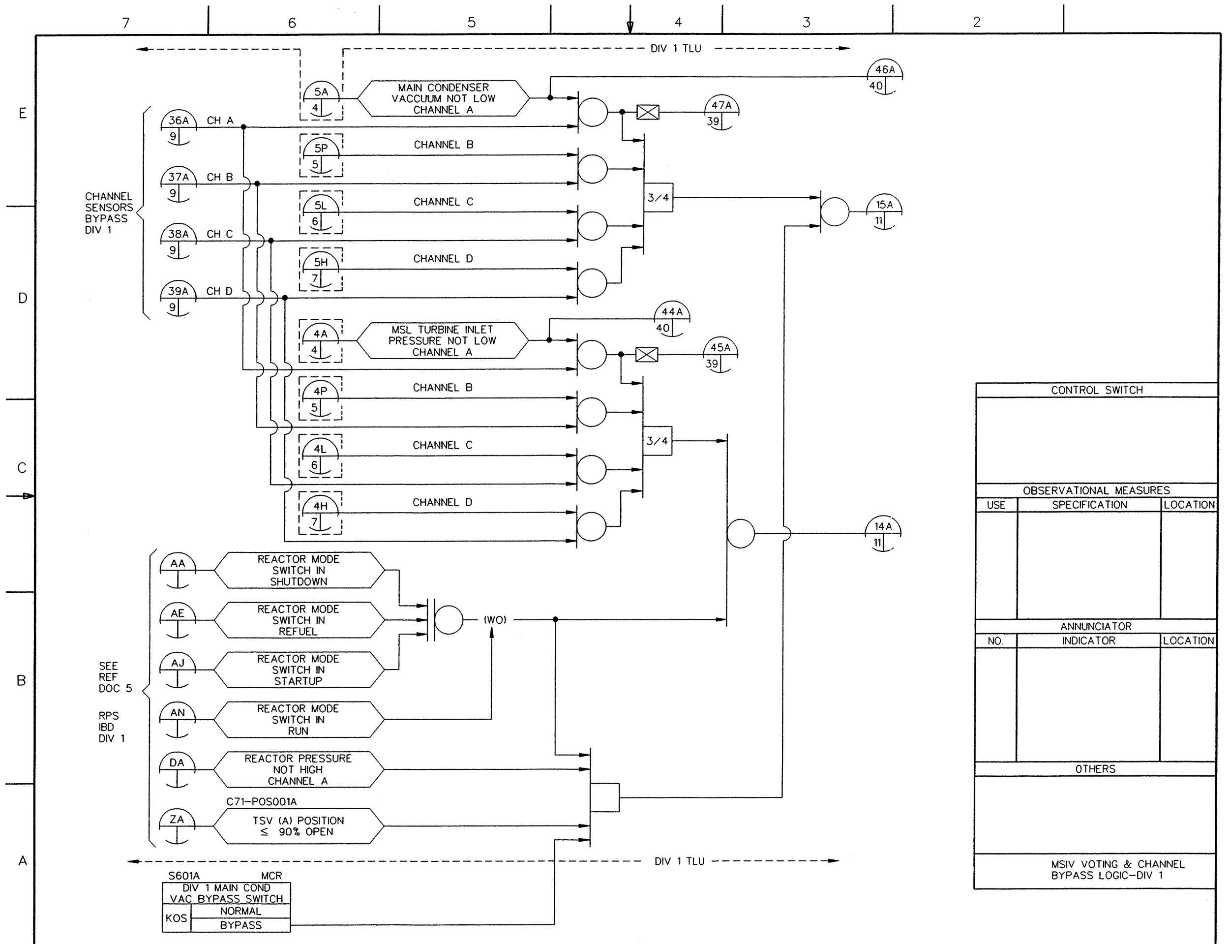
FIGURE 7.3-5 LEAK DETECTION AND ISOLATION SYSTEM IBD (Sheet 10 of 77)
