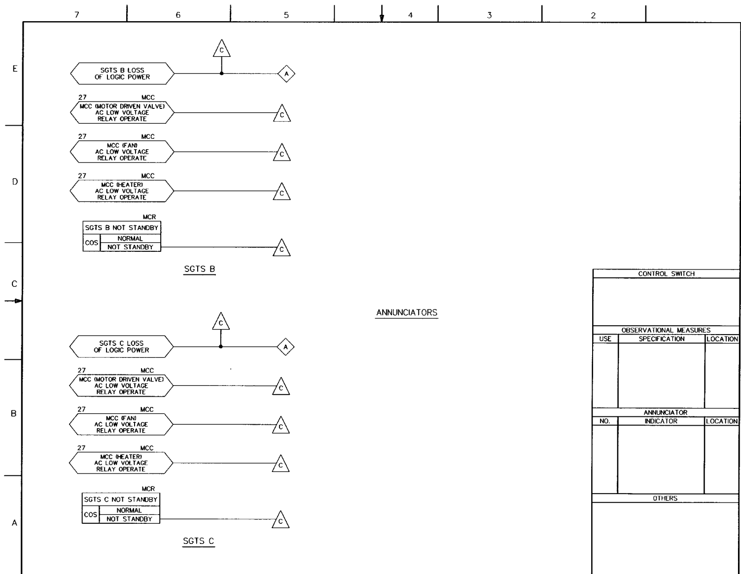
FIGURE 7.3-6 STANDBY GAS TREATMENT SYSTEM IBD (Sheet 8 of 11)
