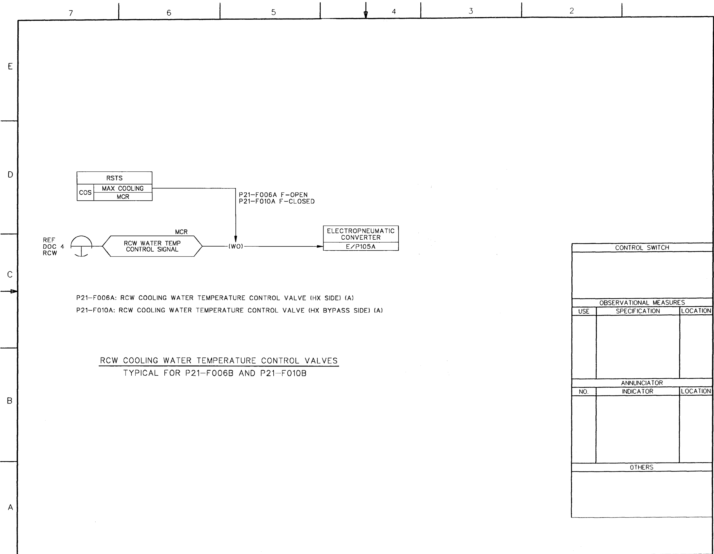
FIGURE 7.4-3 REMOTE SHUTDOWN SYSTEM IBD (Sheet 27 of 27) ABWR DCD/Tier 2 Rev. 0 21-306
