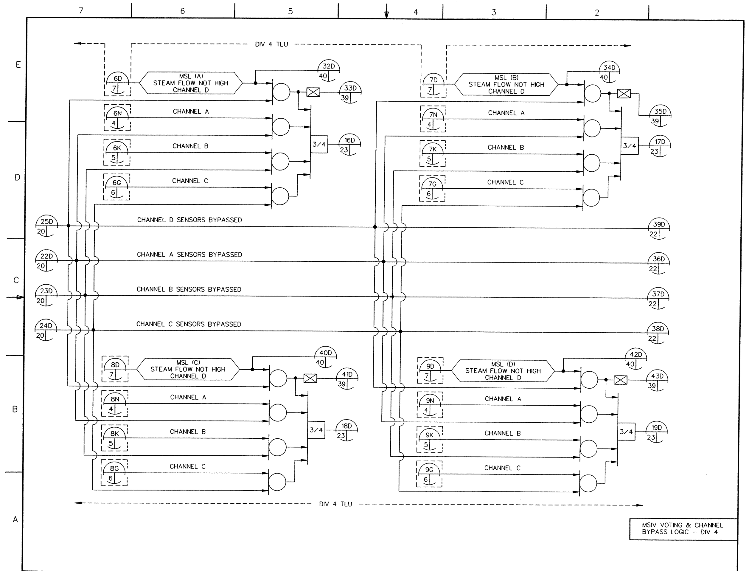
FIGURE 7.3-5 LEAK DETECTION AND ISOLATION SYSTEM IBD (Sheet 21 of 77) ABWR DCD/Tier 2 Rev. 0 21-228.21
