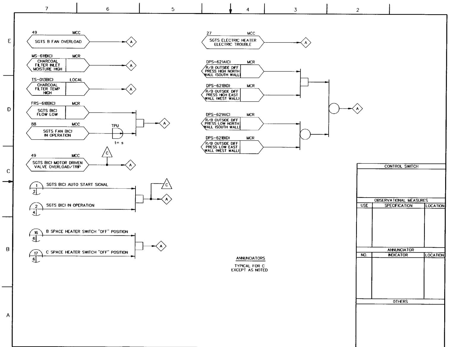
FIGURE 7.3-6 STANDBY GAS TREATMENT SYSTEM IBD (Sheet 10 of 11) ABWR DCD/Tier 2 Rev. 0 21-230
