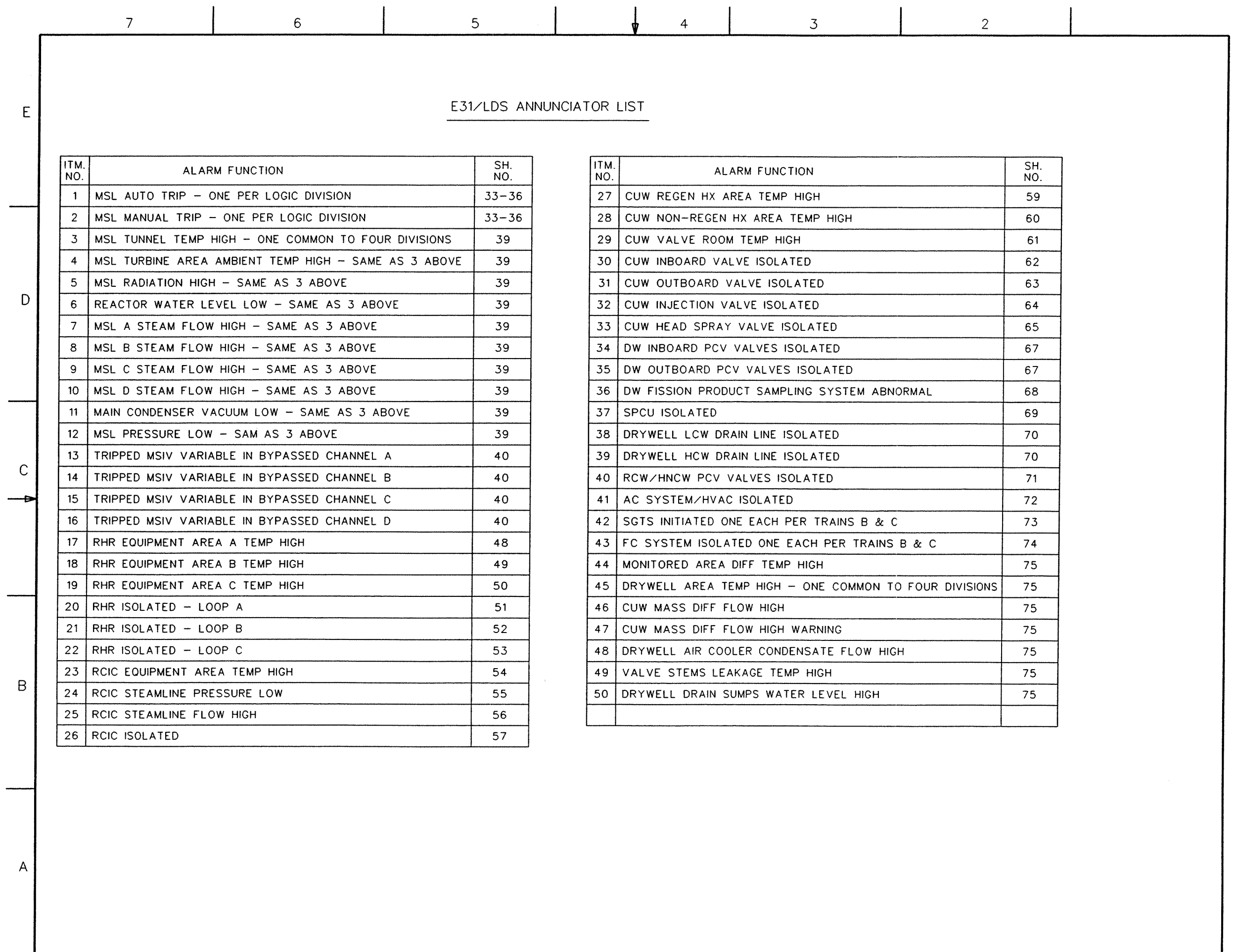
FIGURE 7.3-5 LEAK DETECTION AND ISOLATION SYSTEM IBD (Sheet 3 of 77) ABWR DCD/Tier 2 Rev. 0 21-228.3
