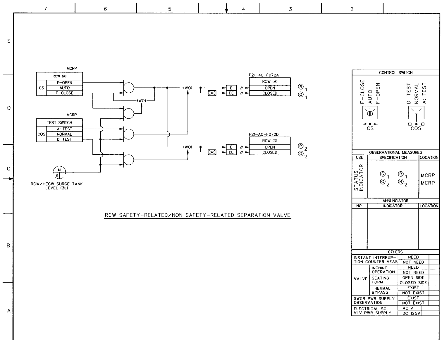
FIGURE 7.3-7 REACTOR BUILDING COOLING WATER/REACTOR SERVICE WATER SYSTEM IBD (Sheet 7 of 19)
