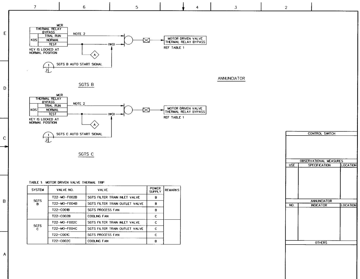
FIGURE 7.3-6 STANDBY GAS TREATMENT SYSTEM IBD (Sheet 9 of 10) ABWR DCD/Tier 2 Rev. 0 21-237
