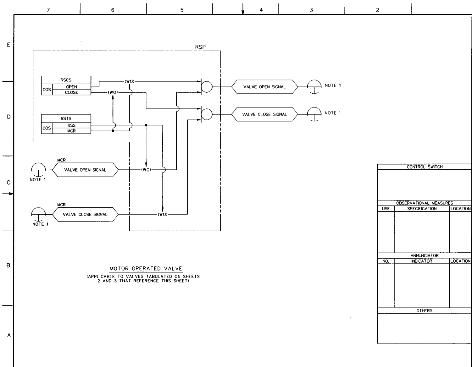
FIGURE 7.4-3 REMOTE SHUTDOWN SYSTEM IBD (Sheet 8 of 27) ABWR DCD/Tier 2 Rev. 0 21-287
