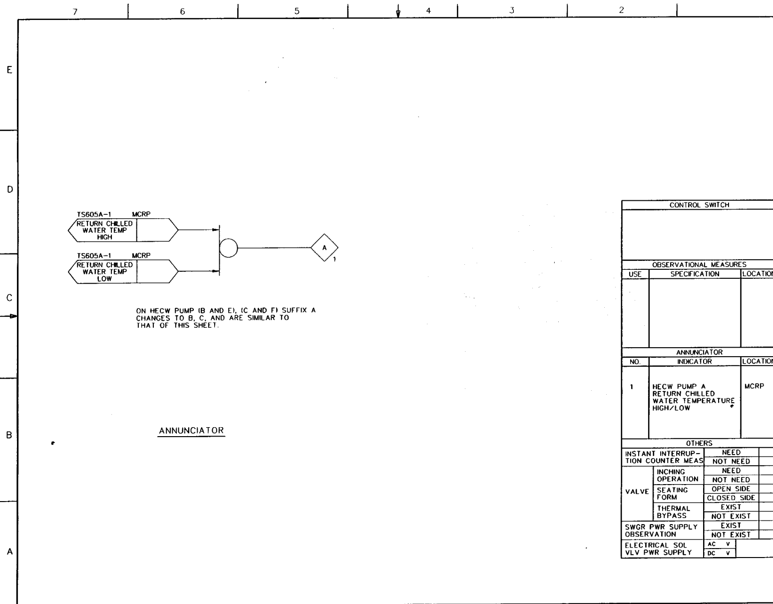
FIGURE 7.3-9 HVAC EMERGENCY COOLING WATER SYSTEM IBD (Sheet 11 of 11) ABWR DCD/Tier 2 Rev. 0 21-269
