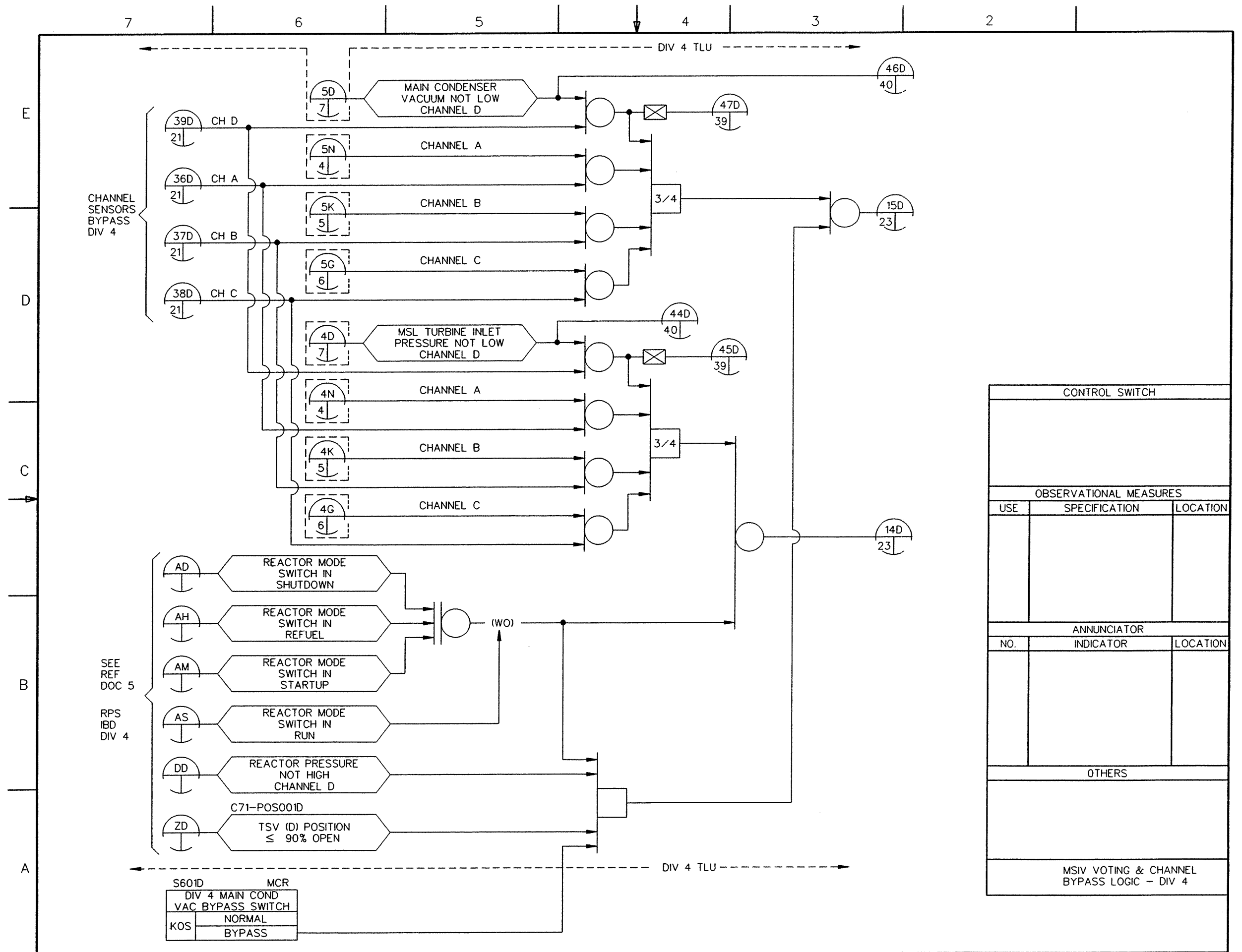
FIGURE 7.3-5 LEAK DETECTION AND ISOLATION SYSTEM IBD (Sheet 22 of 77)
