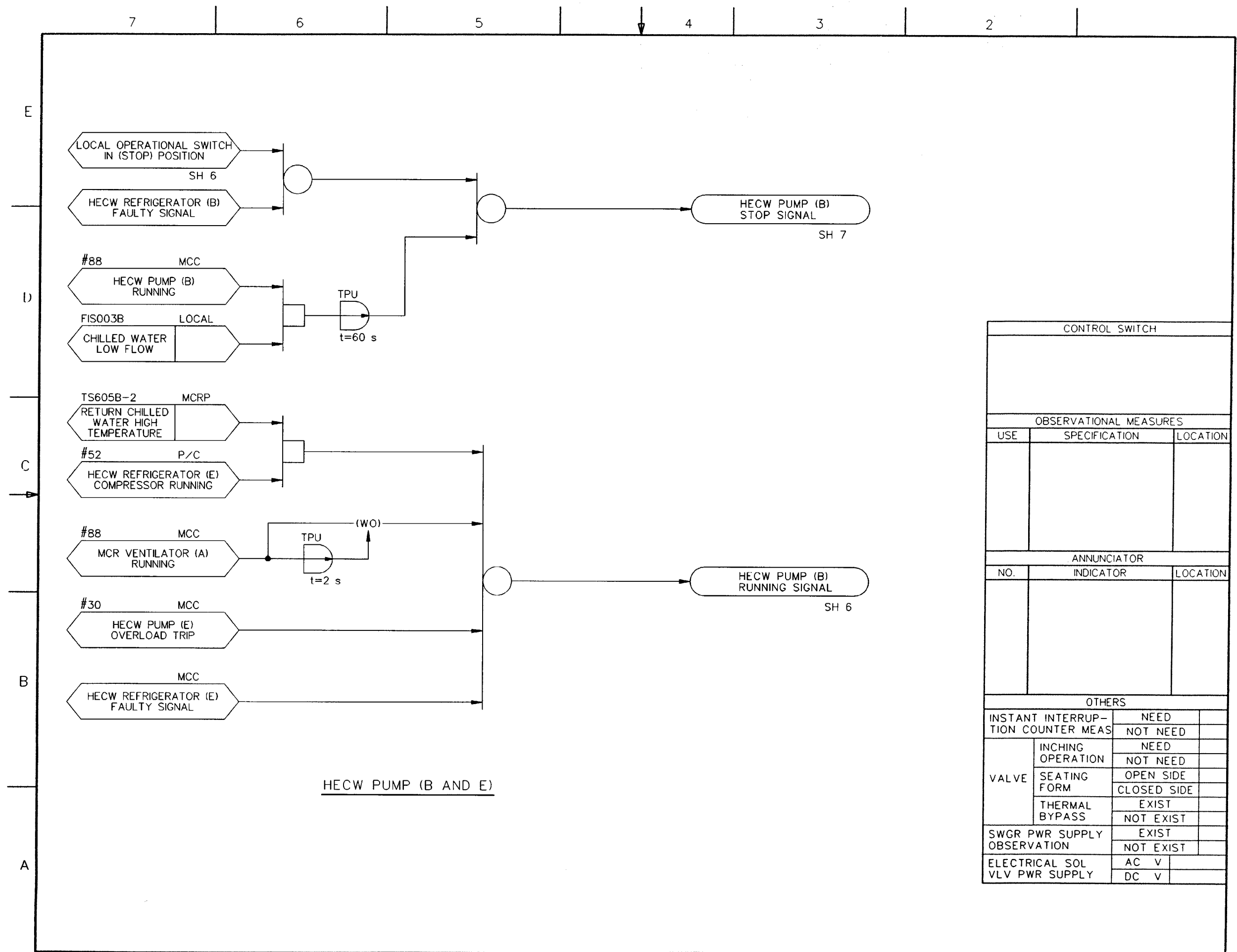
FIGURE 7.3-9 HVAC EMERGENCY COOLING WATER SYSTEM IBD (Sheet 8 of 11) ABWR DCD/Tier 2 Rev. 0 21-266
