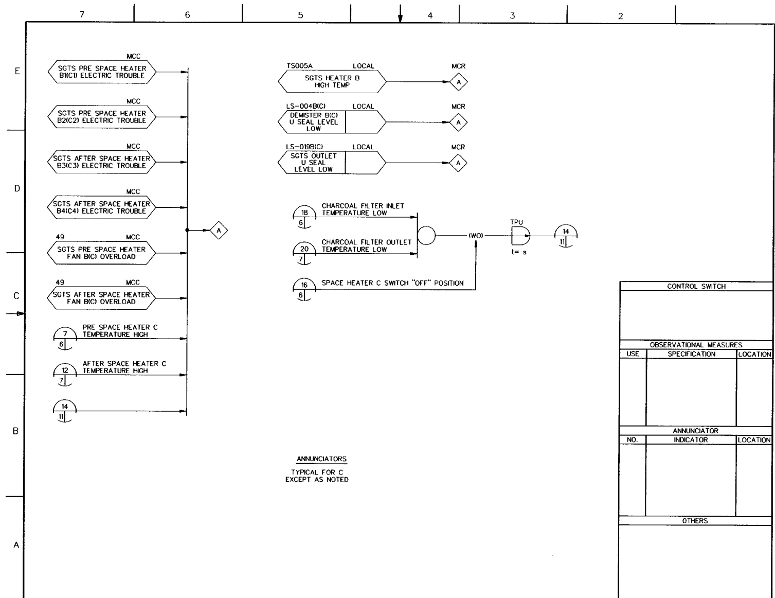
FIGURE 7.3-6 STANDBY GAS TREATMENT SYSTEM IBD (Sheet 11 of 11) ABWR DCD/Tier 2 Rev. 0 21-239
