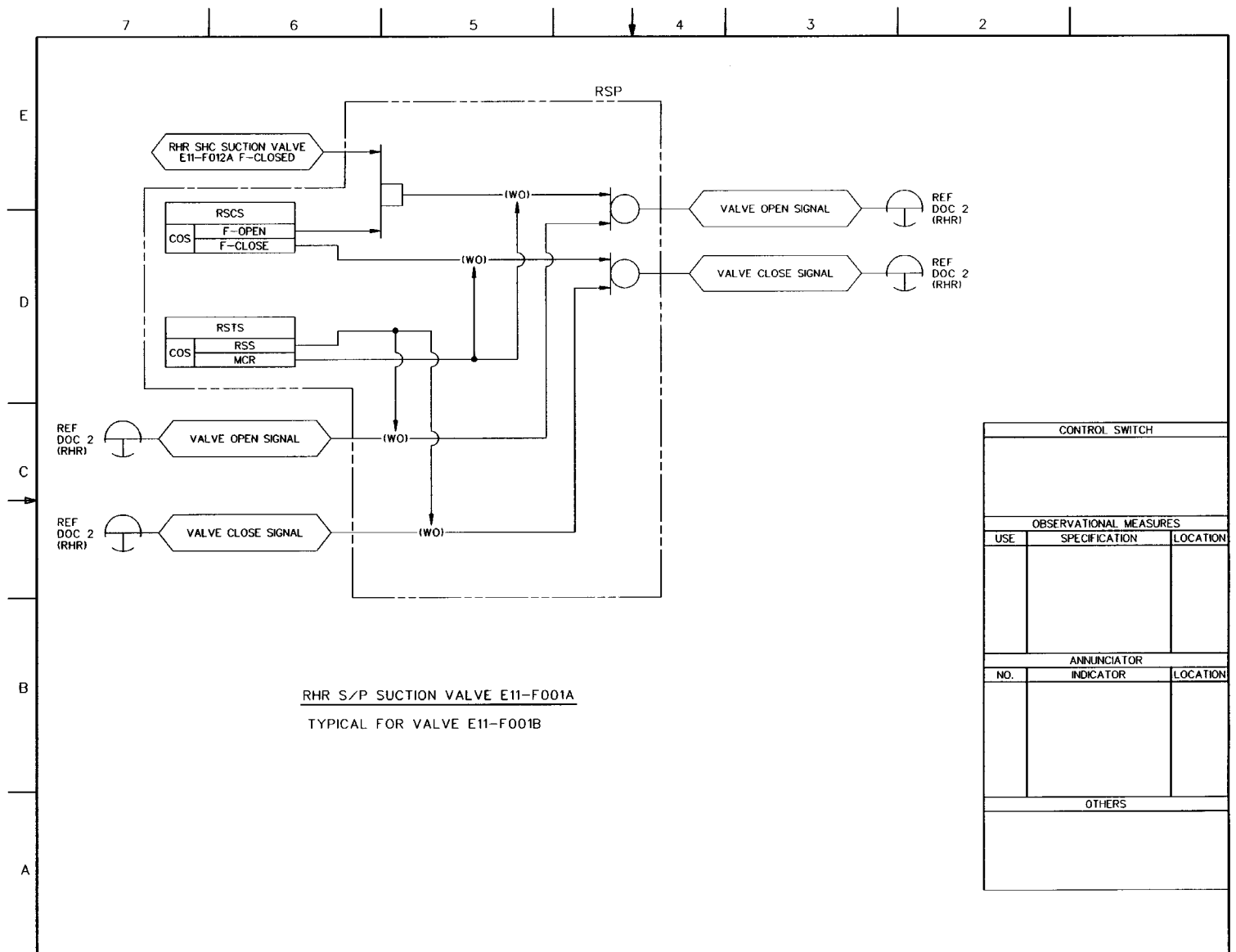
FIGURE 7.4-3 REMOTE SHUTDOWN SYSTEM IBD (Sheet 7 of 27)
