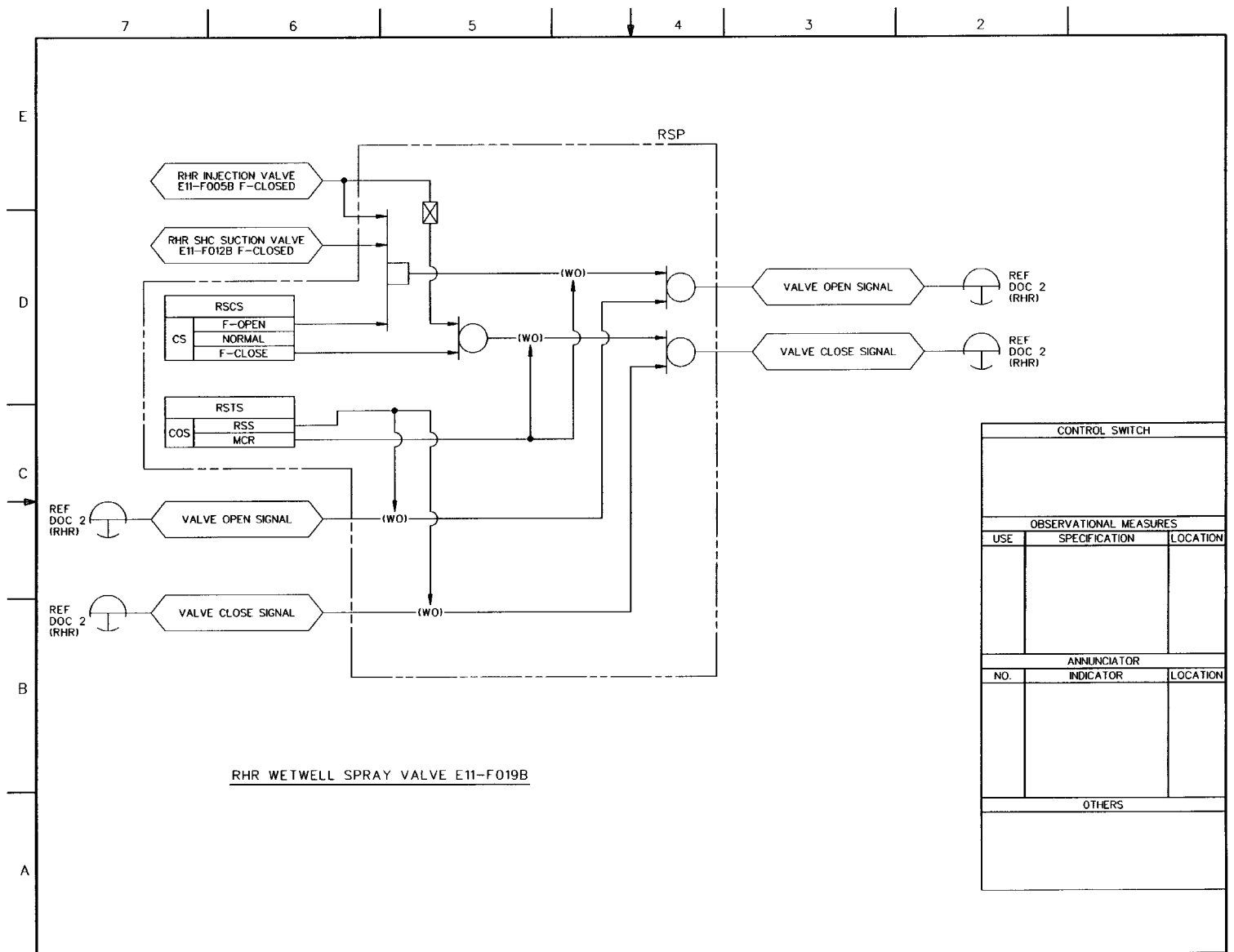
FIGURE 7.4-3 REMOTE SHUTDOWN SYSTEM (Sheet 25 of 27)
